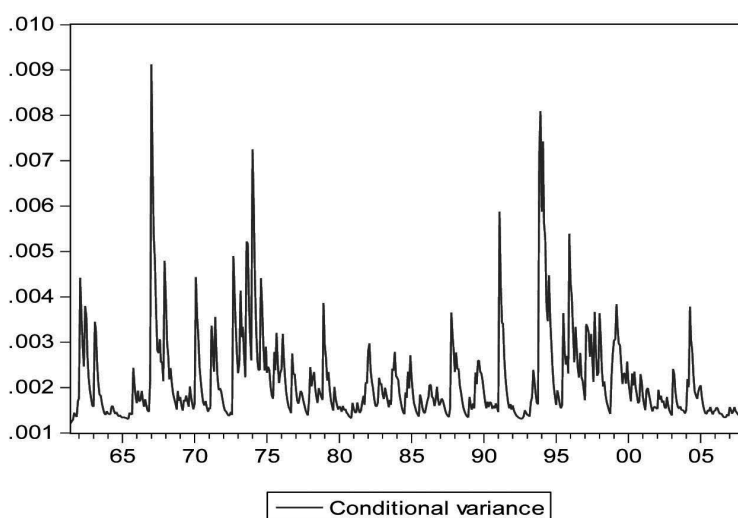
Figure 1 Conditional Variance
